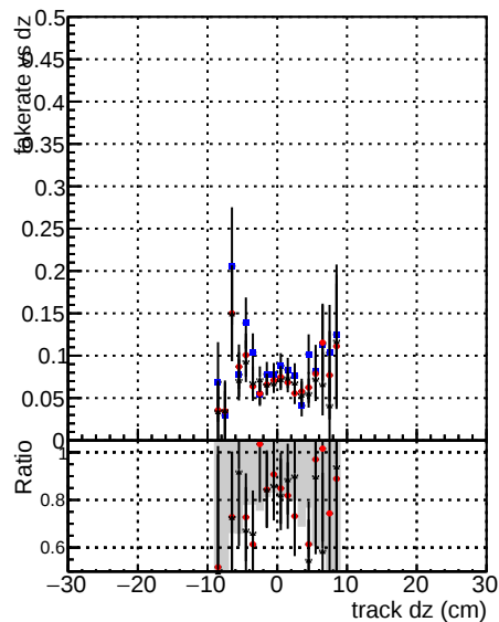
DOMstep3 TT CKF Fake rate vs d —●— —●— Duplicates Rate vs d —●— —●— Pileup rate vs d —●— —●—
