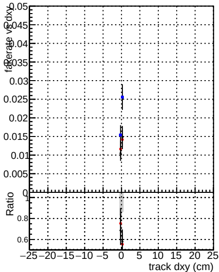
Fake rate vs d —●— DOMstep3 TT CKF —●— DOMstep3 default —●— DOMstep3 default NEWTweight
