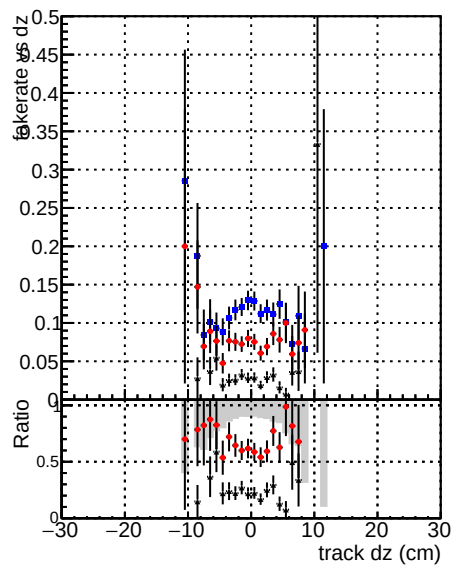
DOMstep3 TT CKF Fake rate vs d blue dots black line Duplicates rate vs d red dots black line Pileup rate vs d blue dots black line Fake rate vs dz blue dots black line Duplicates rate vs dz red dots black line Pileup rate vs dz blue dots black line
