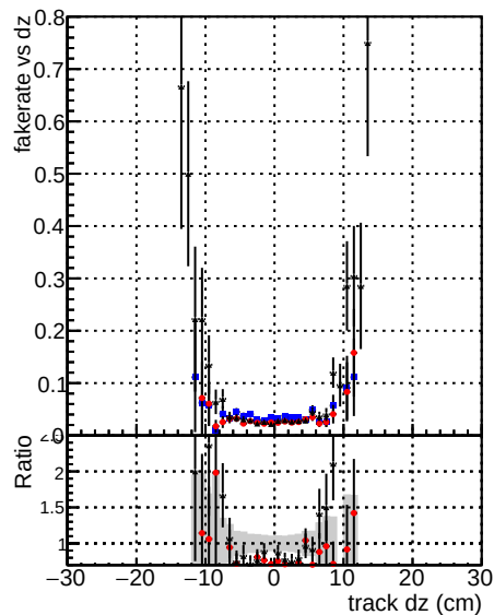
DOMstep3 TT CKF Fake rate vs d blue dots black line Duplicates rate vs d red dots black line Pileup rate vs d black dots black line
