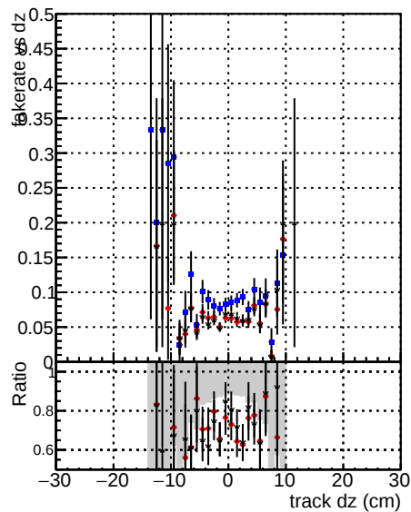
Fake rate vs d DOMstep3 TT CKF default default default NEWTreweight
