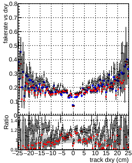
Fake rate vs d DOMstep3 TT CKF DOMstep3 TT default DOMstep3 TT default NEWTweight
