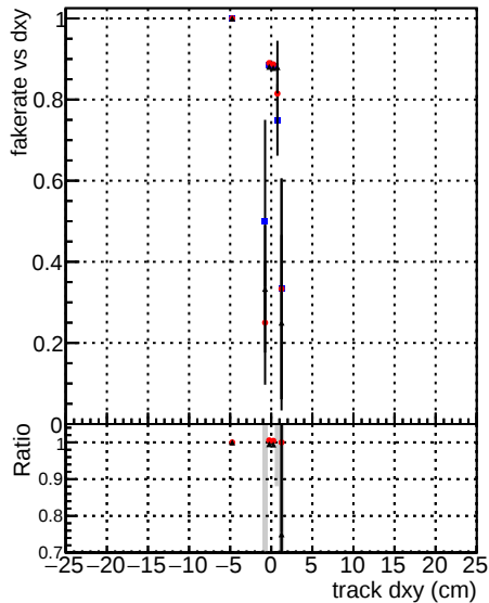
Legend for Fake rate vs dxy, Duplicates Rate vs Dxy, and Pileup rate vs dxy: DOMstep3 (blue circles) TT CKF (black circles) DOMstep3 TT CKF (red circles) default (grey shaded area) NEWT-olddsamples (black crosses)
