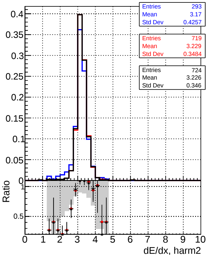
Legend: DQMstep3_TT_CKF (blue line with squares) DQMstep3_TT_default (red line with circles) DQMstep3_TT_defaultNEWT-oldsamples (black line with crosses)
