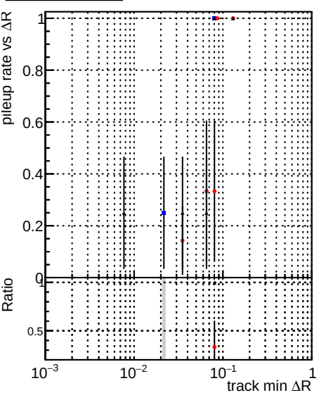
Legend: DOMstep3_TT_CKF (blue dots), DOMstep3_TT_default (red dots), DOMstep3_TT_defaultNEWT-oldsamples (black dots)
