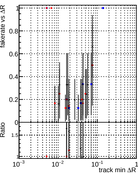
Legend: DOMstep3_TT_CKF (blue dots), DOMstep3_TT_default (red dots), DOMstep3_TT_defaultNEWT-oldsamples (black dots)
