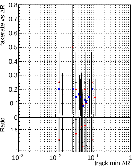
Fake rate vs ΔR(track, jet) Legend: DOMstep3_TT_CKF (blue dots) DOMstep3_TT_default (red dots) DOMstep3_TT_defaultNEWTepo7 (black dots)
