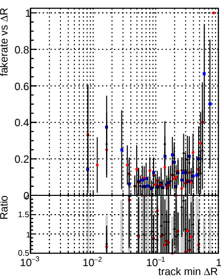
Legend: DQMstep3_TT_CKF (blue dots), DQMstep3_TT_default (red dots), DQMstep3_TT_defaultNEWTepo7 (black dots with error bars)
