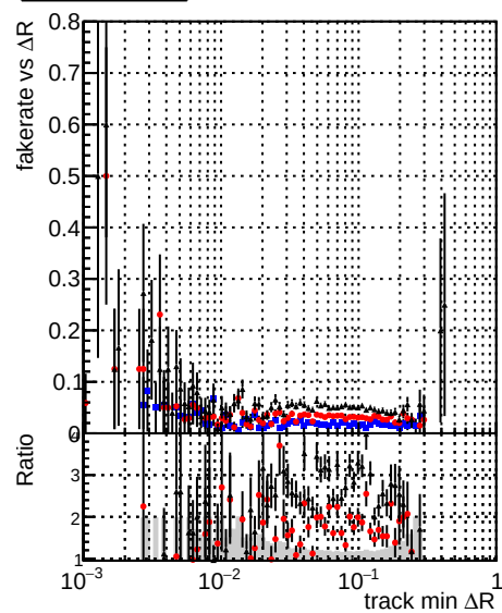
Legend: DOMstep3 TT CKF (blue stars) DOMstep3 TT default (red stars) DOMstep3 TT defaultNEWTepo10 (black stars)
