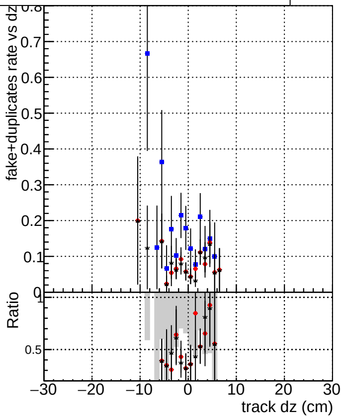
Legend for the bottom plot: DQMstep3_TT_CKF (blue square) DQMstep3_TT_default (red circle) DQMstep3_TT_defaultNEWTepo10 (black triangle)
