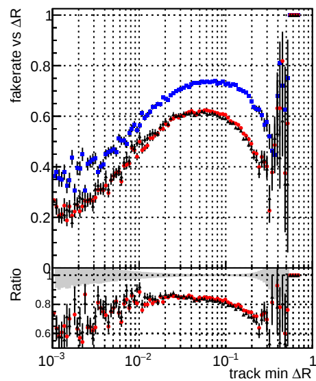
Legend: DQMstep3 TT CKF (blue line with dots) DQMstep3 TT default (red line with dots) DQMstep3 TT defaultNEWTepo10 (black line with dots)
