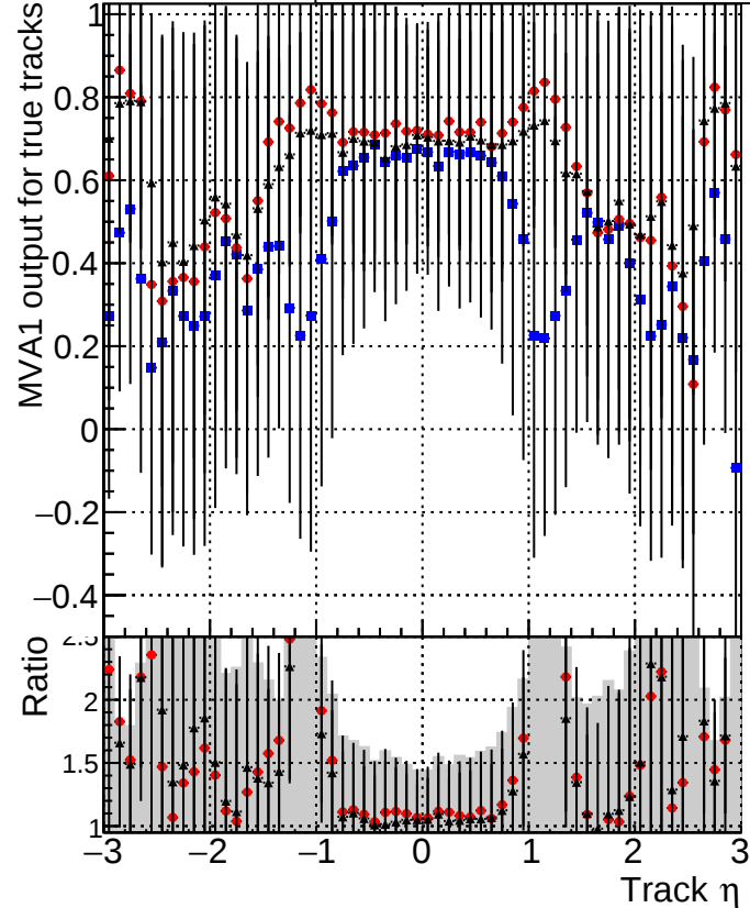
MVA1 of associated tracks (recoToSim) vs. track \eta Legend: DQMstep3_TT_CKF (blue squares) DQMstep3_TT_default (red diamonds) DQMstep3_TT_defaultNEWTepo10 (black stars)
