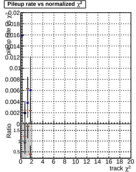
Pileup rate vs. \chi^2
