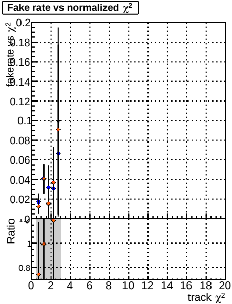
Fake rate vs. DOMster3 DOMster3+GKF DOMster3+GKF+TEC2 Default Less
