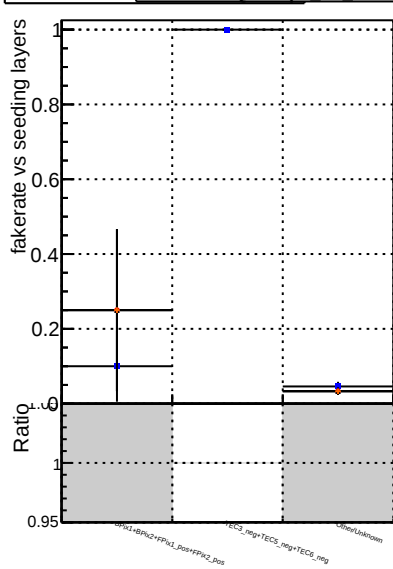
Fake rate vs. DOMster3 DOMster3+GKF DOMster3+GKF+TEC2 Default Less
