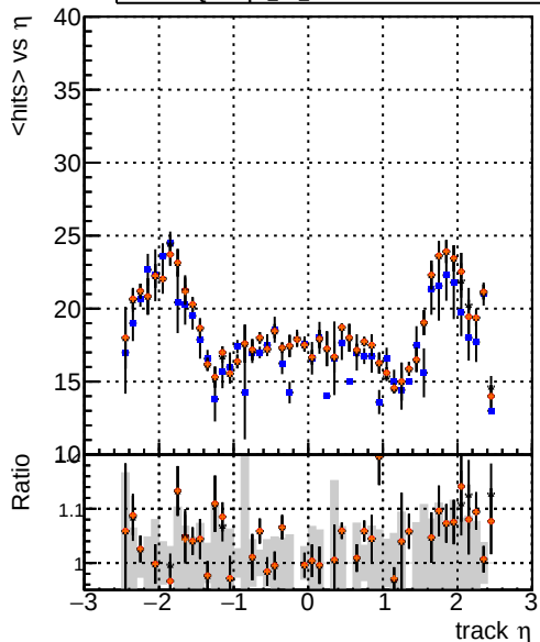
mean hits vs \eta Legend: - DQMstep3 TT CKF (blue line with circles) - DQMstep3 TT default (red line with circles) - DQMstep3 TT ckfPixelLess (black line with circles) - DQMstep3 TT default1 (orange line with circles)
