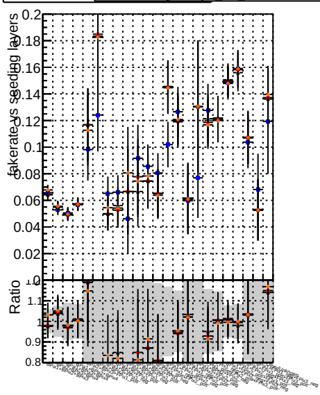
Fake rate vs. DOMstep3 GKF default
