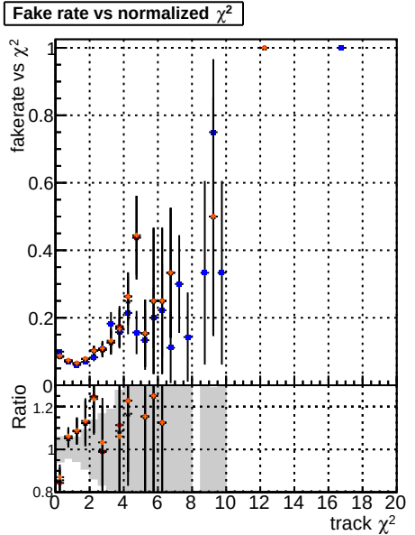
Fake rate vs. DOMstep3 GKF default
