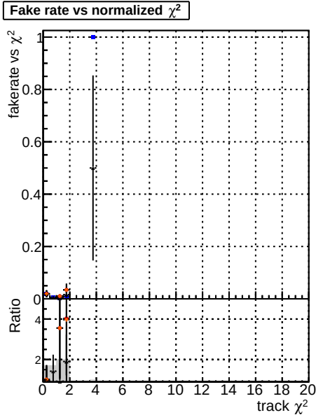
Fake rate vs. Default
