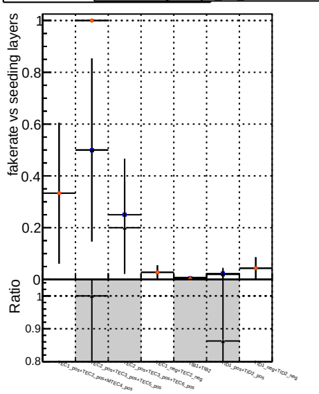
Fake rate vs. Default
