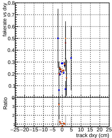
Fake rate vs d DOMstep3 GKF default Less
