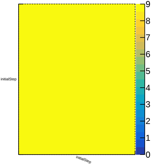
Duplicate tracks: originalAlgo vs originalAlgo
