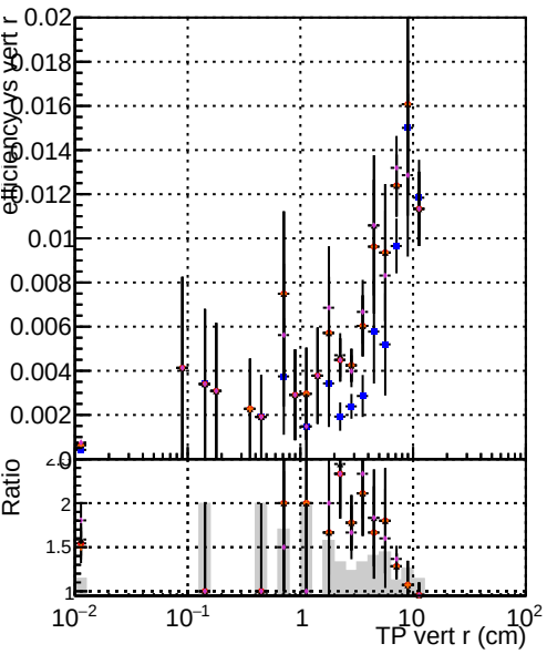
Efficiency vs TP vert r (cm) Legend: DOMstep3 CKF DOMstep3 default DOMstep3 ckfPixelLess DOMstep3 default1 DOMstep3 defaultNEWTOLDSAMPLE
