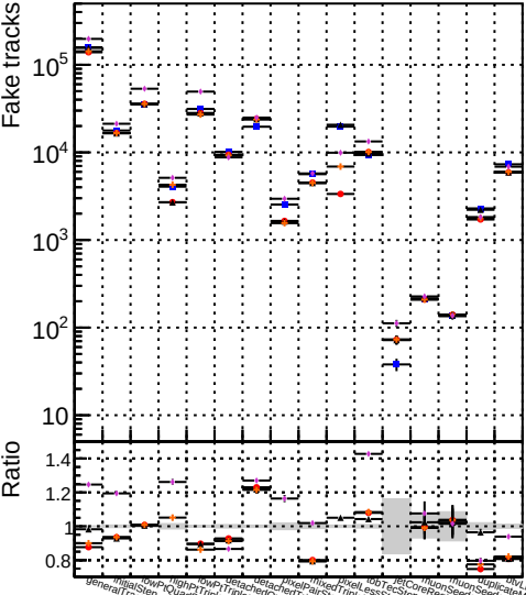
Number Symbol Label 1 Black triangle DOMstep3 TT ckrPixelLess 2 Orange cross DOMstep3 TT default1 3 Purple dot DOMstep3 TT defaultNEWTOLDSAMPLE
