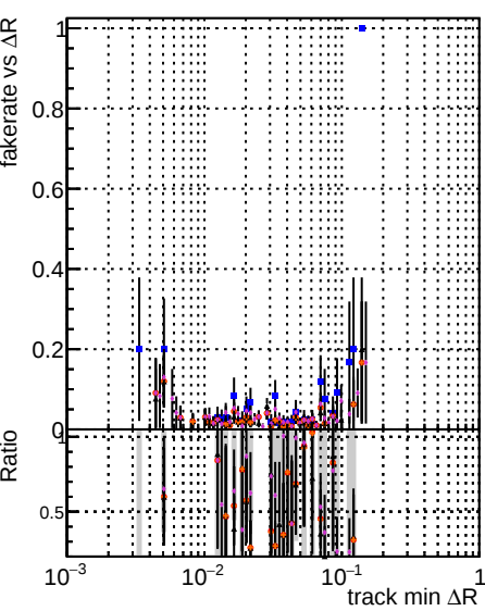
Fake rate vs \Delta R(\text{track}, \text{jet}) DQM M3 M3+GKE M3+GKE+Default M3+GKE+Default+Less NEWTOLD SAMPLE
