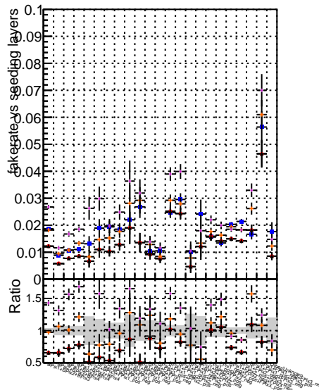
Fake rate vs. DOMstep3 TT GKE default Less NEW TOLDSAMPLE
