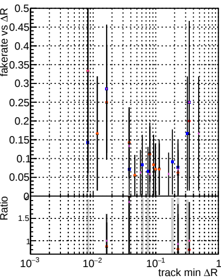
Fake rate vs \Delta R(\text{track, jet}) DQM Meten3 TT GKE default Less NEWTOLDSAMPLE
