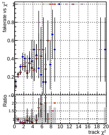
Fake rate vs. \chi^2 layers
