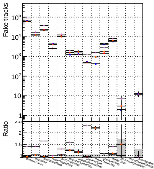
Number Symbol Label ▲ DOMstep3 TT CRIFixLess ● DOMstep3 TT default1 ● DOMstep3 TT defaultNEWTOLDSAMPLE
