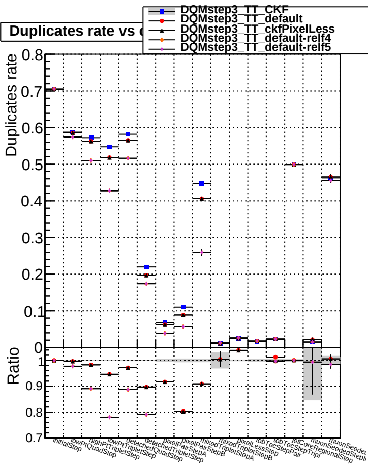
Pileup rate
