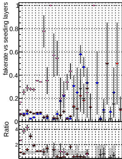
Fake rate vs. DOMestop3 DOMestop3+GKE DOMestop3+GKE+default+retr
