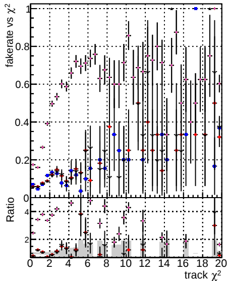
Fake rate vs. DOMestop3 DOMestop3+GKE DOMestop3+GKE+default+retr
