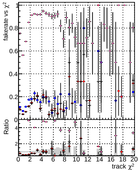
Fake rate vs. DOMestop3 DOMestop3+GKE DOMestop3+GKE+default+less
