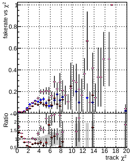
Fake rate vs. DOMeston3 DOMeston2 DOMeston1 default Ratio
