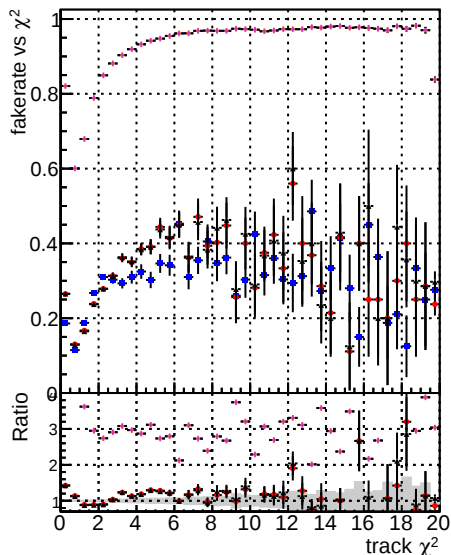
Fake rate vs. DOMestron3 DOMestron3+ DOMestron3+ GKE default rate
