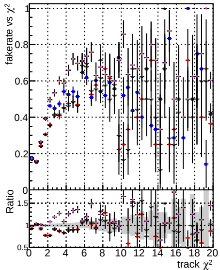
Fake rate vs. DOMestep3 DOMestep3+GKE DOMestep3+GKE+default-retr DOMestep3+GKE+default-retr+less
