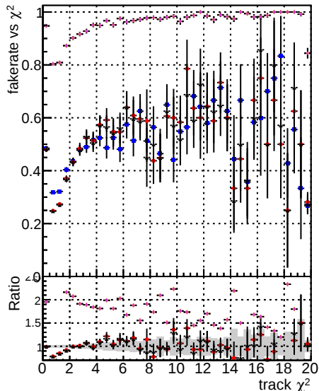
Fake rate vs. DOMestop3 DOMestop3+ DOMestop3- GKF default ratio
