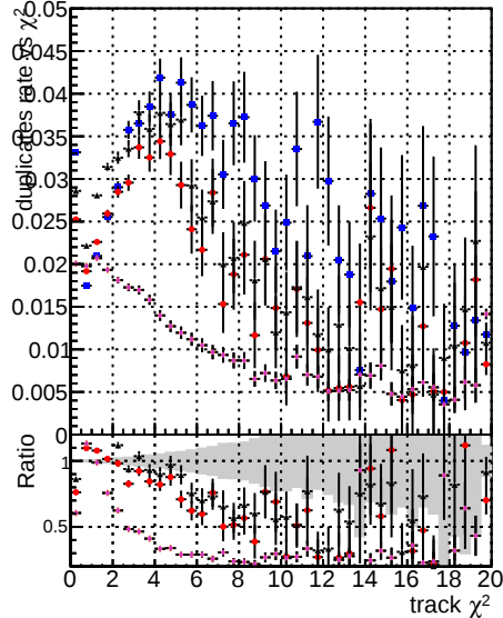
Default NEWTOLDSAMPLE-relf4
