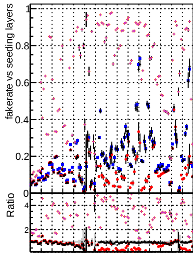
Fake rate vs. DOMstep3 DOMstep3+GKE DOMstep3+GKE+PileupLess
