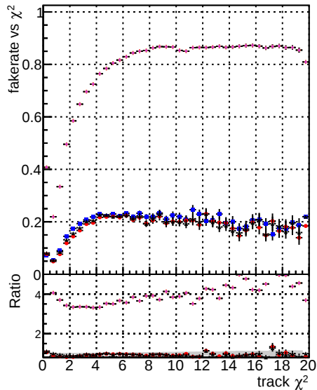
Fake rate vs. DOMstep3 DOMstep3+GKE DOMstep3+GKE+PileupLess
