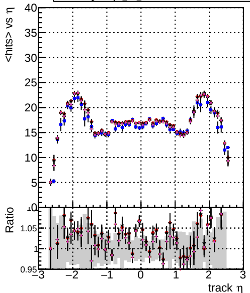
mean hits vs \eta DOMstep3 CKF DOMstep3 default DOMstep3 CKFPixelLess DOMstep3 default-relf4 DOMstep3 default-NEWTOLDSAMPLE-relf4
