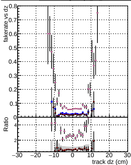
Model Fake rate DOMstep3 ~0.15 TT GKE default ~0.15 TT GKE full ~0.25 TT GKE less ~0.05 TT default NEWT ~0.15
