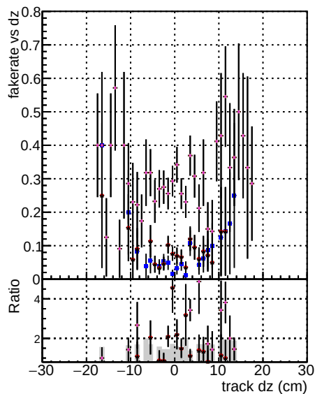
Model Fake rate DGM step 3 ~0.8 TT GKE ~0.6 TT default ~0.5 TT GKE default ~0.4 TT GKE default less ~0.3
