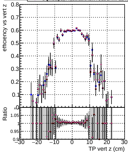
Efficiency Series Configuration ~0.95 DOMstep3 TT ckIPixelLess ~0.90 DOMstep3 TT default-rlf4 ~0.85 DOMstep3 TT defaultNEWTOLDSAMPLE-rlf4
