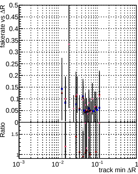
Fake rate vs ΔR(track, jet) for various models: DOM, Meten3, TT, GKE, default, and others. The legend also includes TOLD, SAMPLE, reif4, and NEW.
