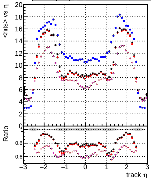
mean hit DOMstep3 TT CKF DOMstep3 TT ckfPixelLess DOMstep3 TT default-relf4 DOMstep3 TT default-NEWTOLDSAMPLE-relf4
