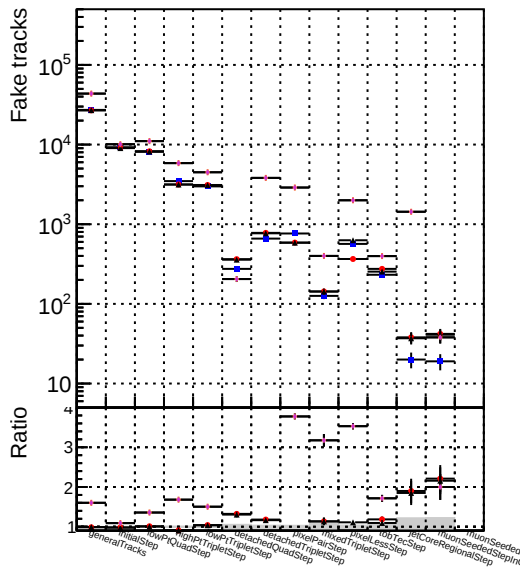
Number Symbol Label ▲ DOMstep3 TT CKIPixelLess + DOMstep3 TT default-rlf4 ◆ DQMstep3 TT defaultNEWTOLDSAMPLE-rlf4
