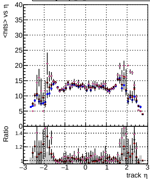
mean hits vs \eta DOMstep3 CKF DOMstep3 default DOMstep3 ckPixelLess DOMstep3 default-relf4 DOMstep3 default-NEWTOLDSAMPLE-relf4
