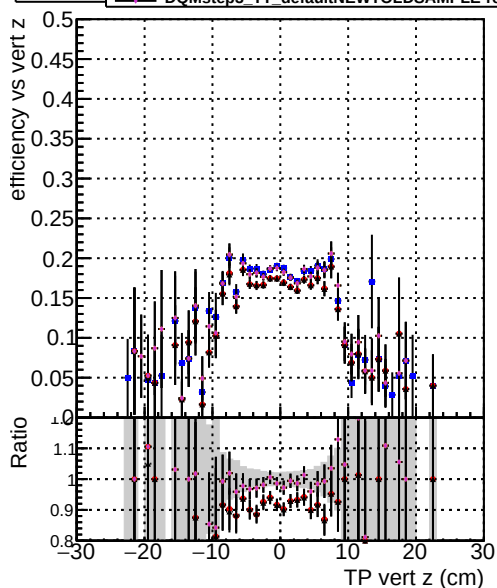
Efficiency DOMstep3 TT cktPixelLess DOMstep3 TT default-rlf4 DOMstep3 TT defaultNEWTOLDSAMPLE-rlf4
