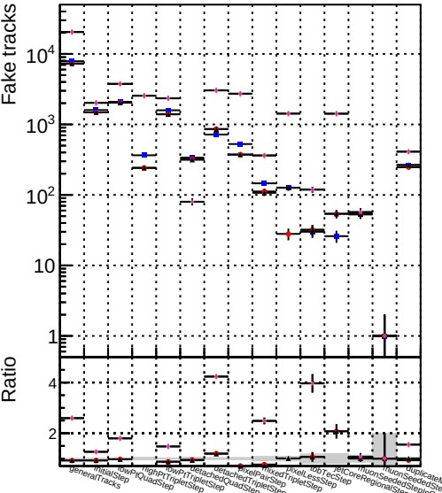
Number Symbol Parameter ▲ DOMstep3 TT ckrPixelLess ● DOMstep3 TT default-relu4 ◆ DOMstep3 TT defaultNEWTOLDSAMPLE-relu4
