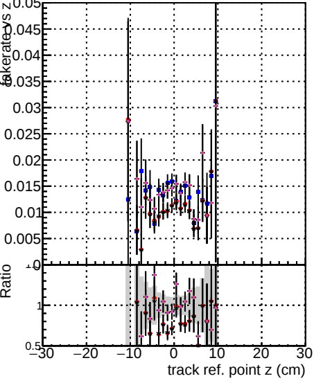
Fake rate vs v DOMstep3 TT GKF DOMstep3-default DOMstep3-CellLess DOMstep3-NEW TOLDSAMPLE-relf4
