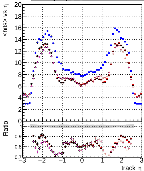
mean hits > \eta
