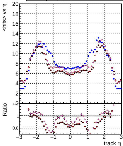
Legend: DOMstep3 TT CKF, DOMstep3 TT default, DOMstep3 TT ckPixelLess, DOMstep3 TT default-relf4, DOMstep3 TT defaultNEWTOLDSAMPLE-relf4 mean hits
